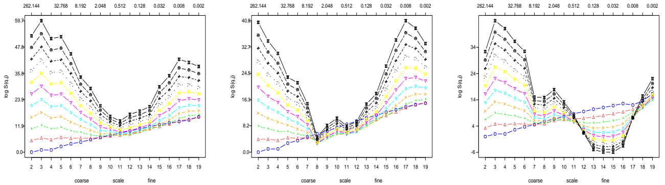
Figure 11: Impact of ACK compression on local scaling – traffic to and from server 2 according to its protocol components. From left: all packets, ACKs only, and TCP data only; (CROSSBELL, 400 MODEM NODES, PARETO 2).
