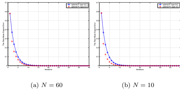
Figure 4: Comparison of optimal learning performance
