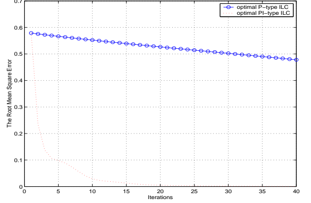
Figure 2: Comparison of optimal P-type and PI-type ILC for H_1(z)
