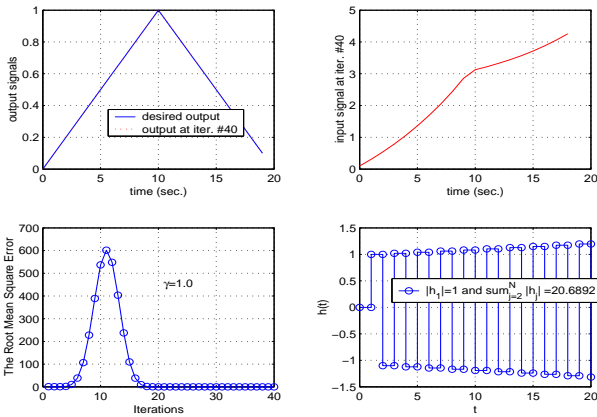
Figure 1: P-type ILC result for slightly unstable highly oscillatory system H_1(z)
