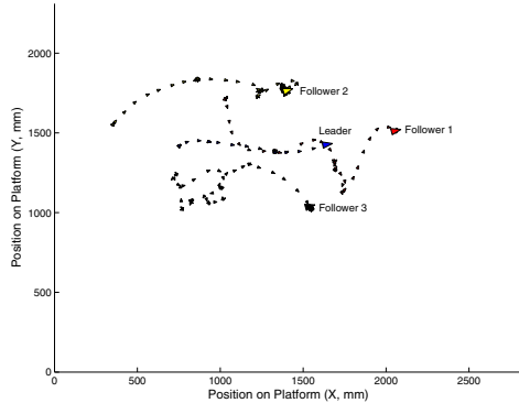
(b) Formation moves to right.
