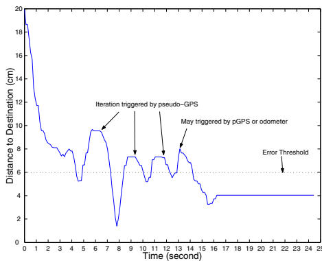
(b) Position error in the movement
