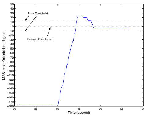
Fig. 6. Spin-in-place under iterative control.
